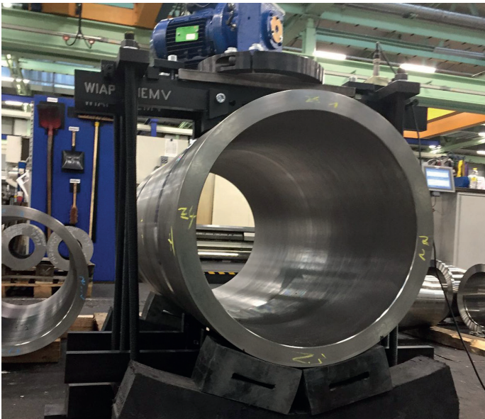
Duplex-Rohr-Test.
